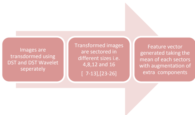
Figure 1 Steps to generate the feature vectors
