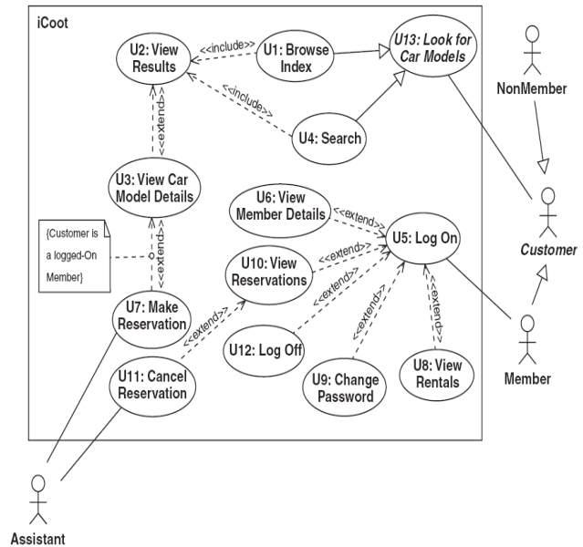
Figure 2: A use Case Diagram
