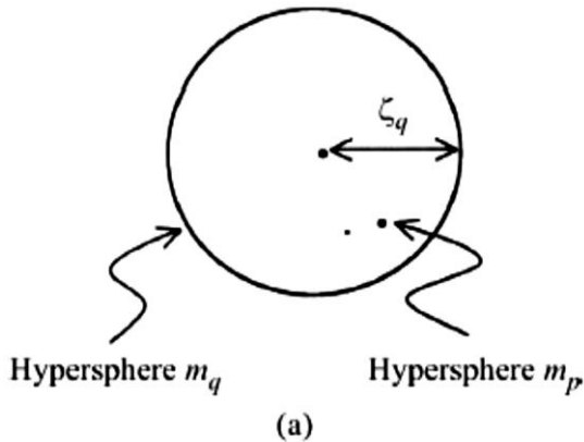
Figure 4. (a) Status of hypersphere before removing an overlap in step 3.
