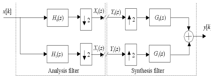
Figure 2: A block diagram of the QMF filter architecture
