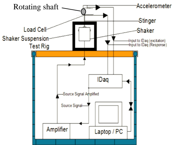
A. The conceptual design show method of the outcome results using electromagnetic Shaker test.
