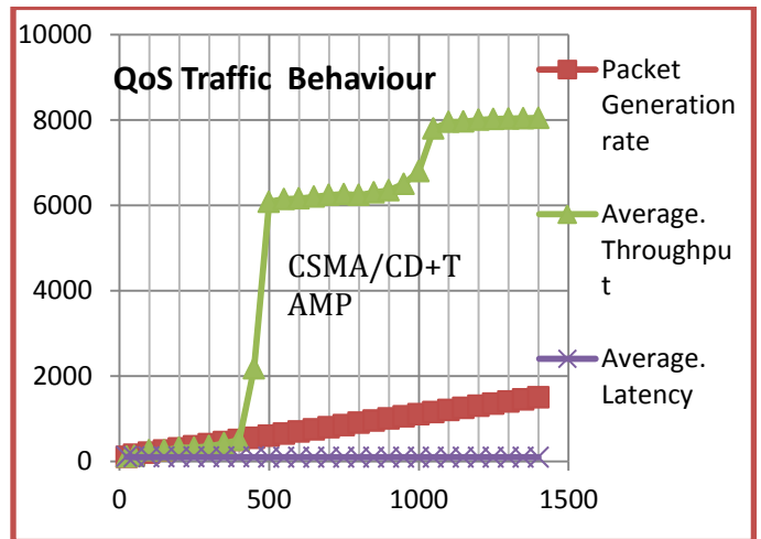
Figure 14. A plot of Reengineered DCN QoS Traffic Behaviour
