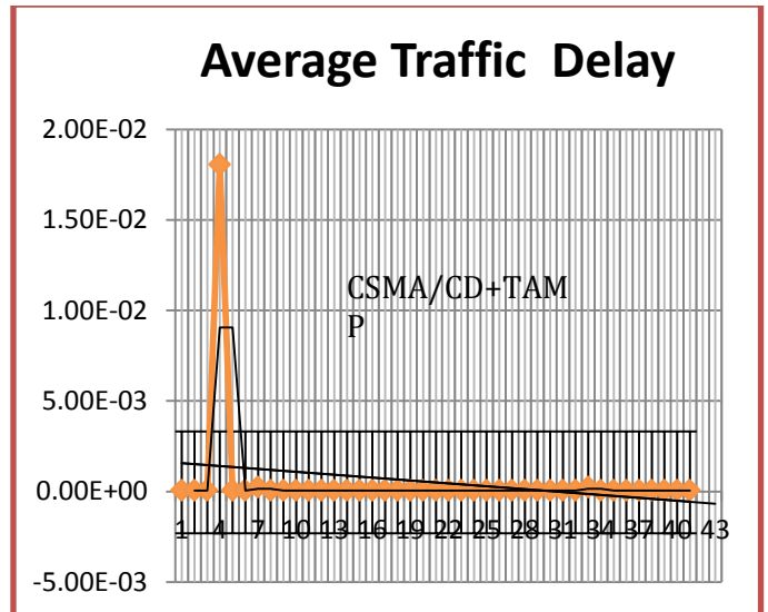
Figure 13. A plot of Reengineered DCN Average Traffic Delay
