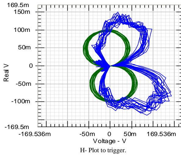
Figure 3. Experimental orbit analysis fundamentals behaviour for key-phasor;
