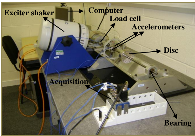
A. Rotor Rig setup for the modal testing.
