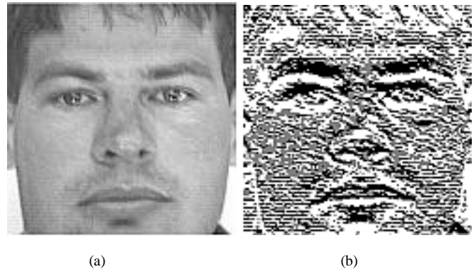
Figure 2. (a). Grayscale image; (b) Vertical gradient image.
