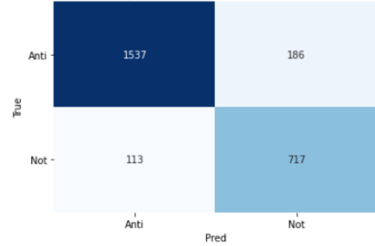
Fig. 8. Confusion Matrix using Tri-gram Level TF-IDF with SVM for Non-Balanced Arabic Dataset.
