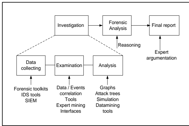
Fig. 2. Cybercrime process
