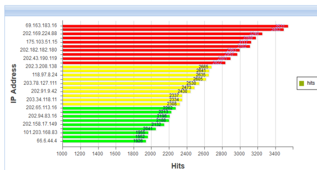
Fig. 8. The result of the clustering process step NFAT machine.
