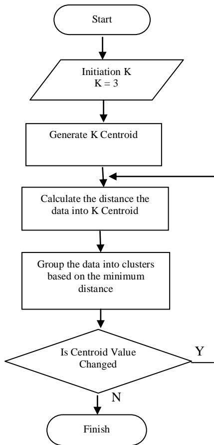
Fig. 5. Flowchart k-means clustering algorithm for grouping log.
