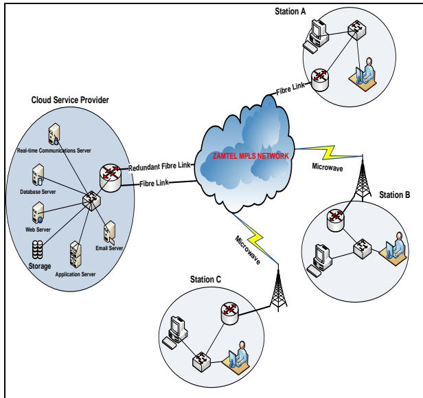
Fig. 4. Proposed system architecture.
