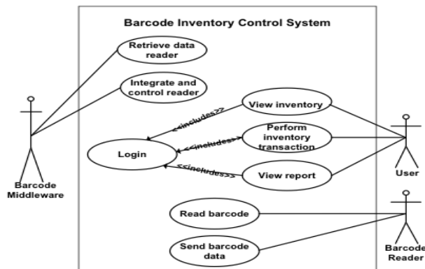
Fig. 5. Use case diagrams.
