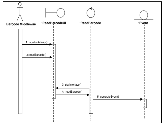
Fig. 6. Sequence diagram.
