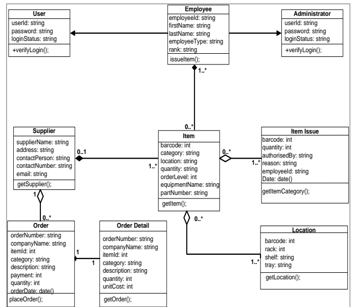
Fig. 7. Class diagram.
