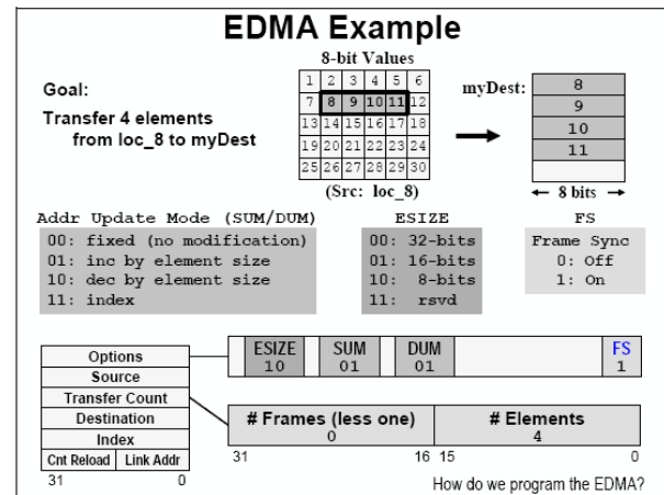
Fig. 10. EDMA example.
