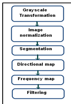
Fig. 1. Pre-processing steps.
