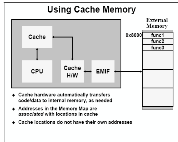
Fig. 13. Using cache memory for C6000 DSP.
