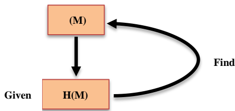
Fig. 3. Preimage resistance.
